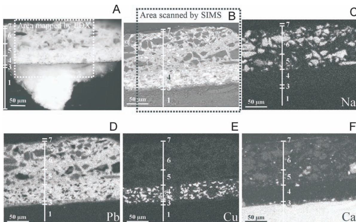
Fig. 2.3 (A) Light microscopic image of paint cross-section van der Weyden (A166/1b) with a square indicating the measured area for the backscattered image and X-ray maps; (B) backscattered electron (BSE) image of paint cross-section van der Weyden (A166/1b) with a square outlining the scanned SIMS area; (C-F) X-ray maps of sodium (C), lead (D), copper (E) and calcium (F).
