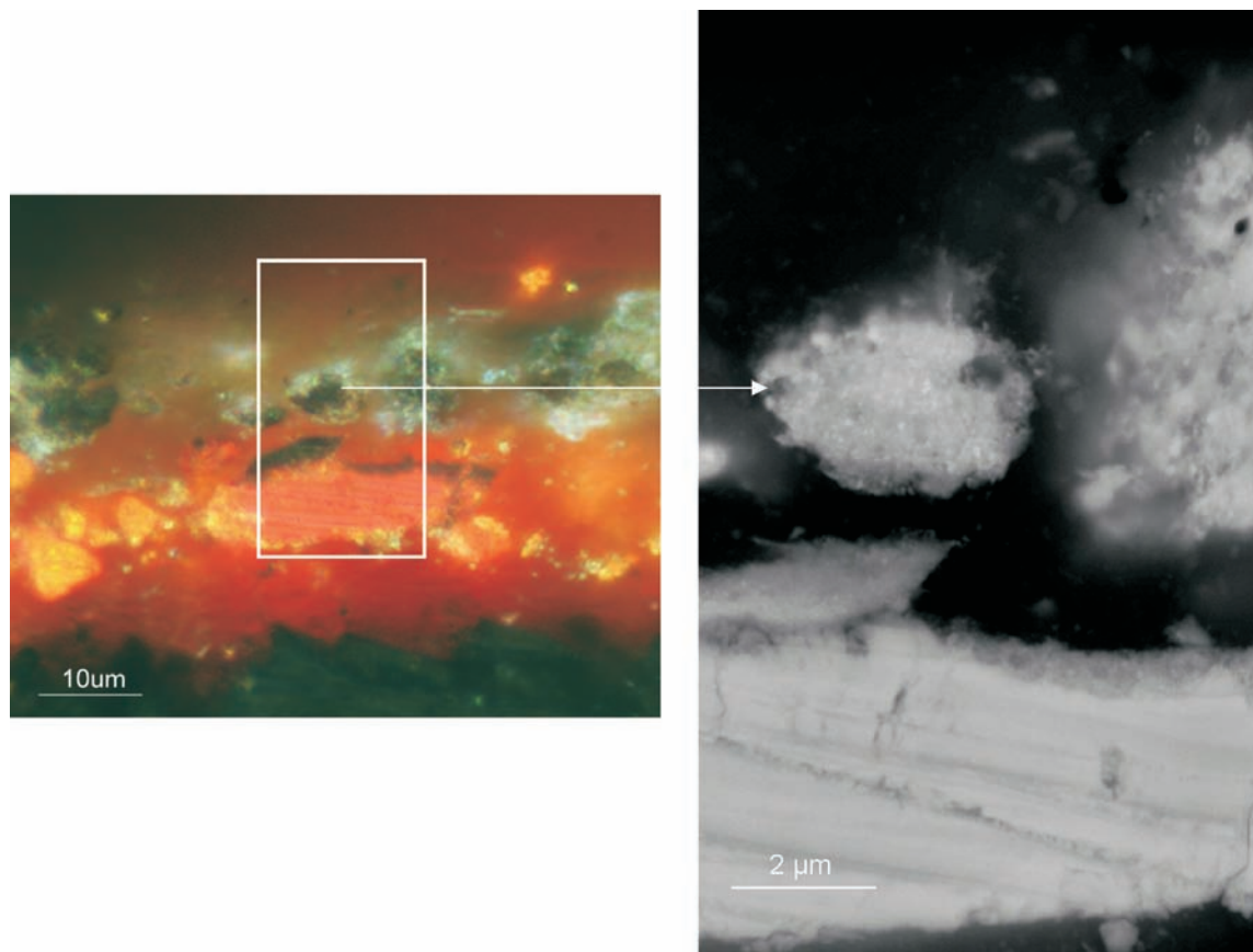
Supplementary Fig. 4.1 The BSE-image visualises a black particle containing hotspots of smaller than 100 nm. These hotspots are nanoparticles of metallic mercury.
