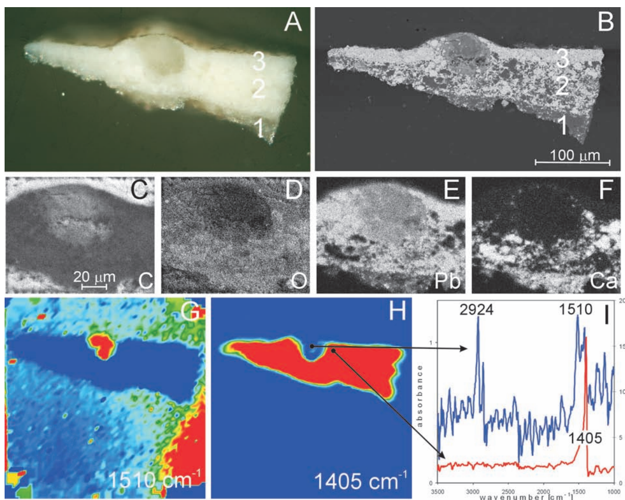
Fig. 5.5A-I A large lead soap aggregate is visible in the white light microscopic image (A) of a paint cross-section originating from the preprimed canvas used by Frederic E. Church (1826-1900). The BSE-image and X-ray maps of carbon (CK) (C), Oxygen (OK) (D), lead (PbM) (E) and calcium (CaK) (F) expose the particle and elemental distribution. FTIR images show lead carboxylates (G) in the aggregate and carbonates (H) in the rest of the paint sample. Two FTIR spectra derived from a single point in the aggregate and in the paint matrix (I).
