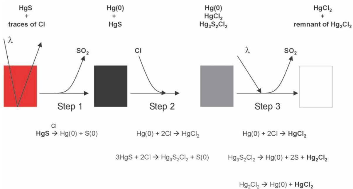
Fig. 4.7 Scheme of the proposed mechanisms of the degradation process of the red vermilion into a black and finally a white product.
