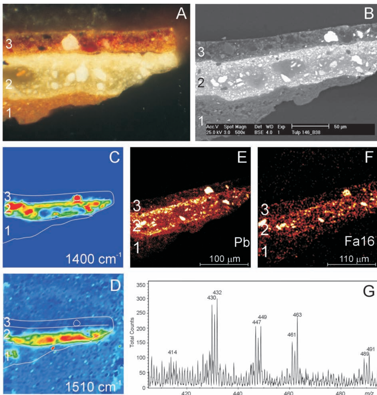
Fig. 5.1 Analytical imaging studies of paint cross-section MH146/B38 taken from 'The Anatomy Lesson of Dr. Nicolaes Tulp' by Rembrandt van Rijn (1632). White light microscopic image (A) and backscattered electron image (BSE-image) (B) reveal the layer buildup and granulometry. FTIR images represent carbonate carbonyl groups at 1400\text{ cm}^{-1} (C) and lead carboxylates at 1510\text{ cm}^{-1} (D) (red represents high and blue low intensity). An outline illustrates the three layers and the circle in layer 3 is indicative for the large lead white particle in this layer. SIMS-images represent lead (+; m/z 206-208) (E) and deprotonated palmitic acid (-; m/z 255) (F). A part of the positive SIMS spectrum presents \text{Pb}_2\text{O} at m/z 426-432, \text{Pb}_2\text{O}_2\text{H} at m/z 443-449, \text{PbOOC}(\text{CH}_2)_{14}\text{CH}_3 at m/z 461-463 and \text{PbOOC}(\text{CH}_2)_{16}\text{CH}_3 at m/z 489-491 (G).
