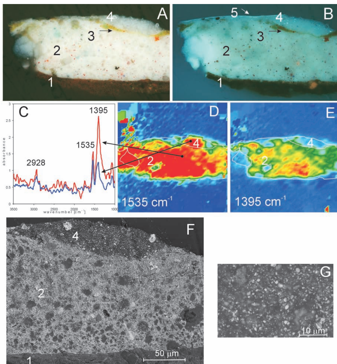
Fig. 5.8A-G Paint cross-section F347-1 originating from 'Impasse des deux frères and Moulin de Poivre' by Vincent van Gogh (1887) is depicted in the light microscopic images in white light (A) and UV (B). Two reflection FTIR spectra derived from a single point in layer 2 and layer 4 (C). FTIR images of metal carboxylates at 1535\text{ cm}^{-1} (D) and carbonates at 1395\text{ cm}^{-1} (E) reveal a saponified layer 2 and 4. BSE-image (F), (detail of layer 4 (G)) reveal the middle part of the paint cross-section.
