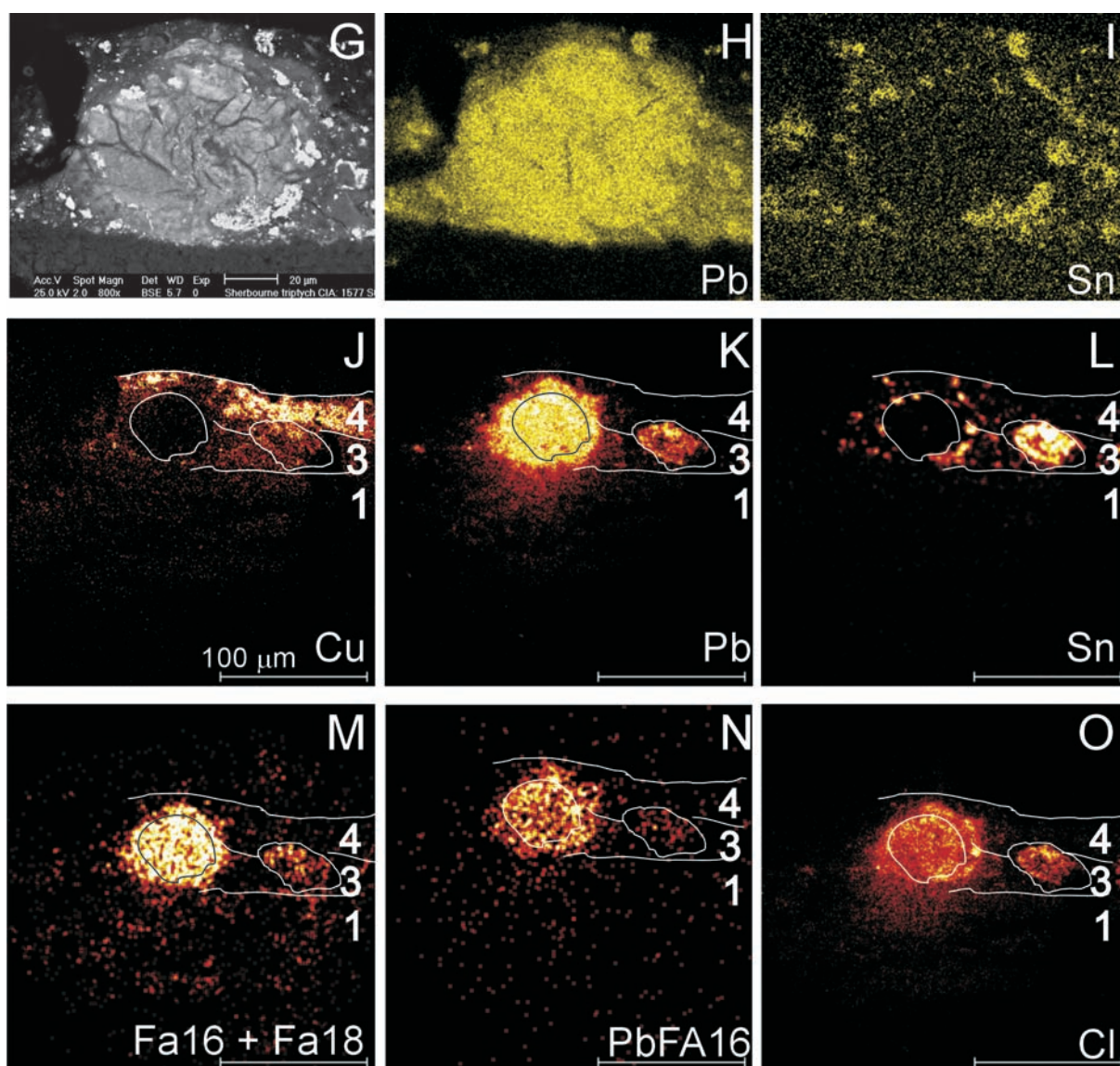
Fig. 5.6 G-O BSE-image (G) and X-ray maps of lead (PbM) (H) and tin (SnL) (I) indicate the large lead soap aggregate. SIMS-images represent copper (+; m/z 63) (J), lead (+; m/z 208) (K), tin (+; m/z 52) (L), the sum of deprotonated palmitic and stearic acid (-; m/z 255 + m/z 283) (M), palmitic acid lead soap (+; m/z 461-463) (N) and chloride (-; m/z 35) (O).
