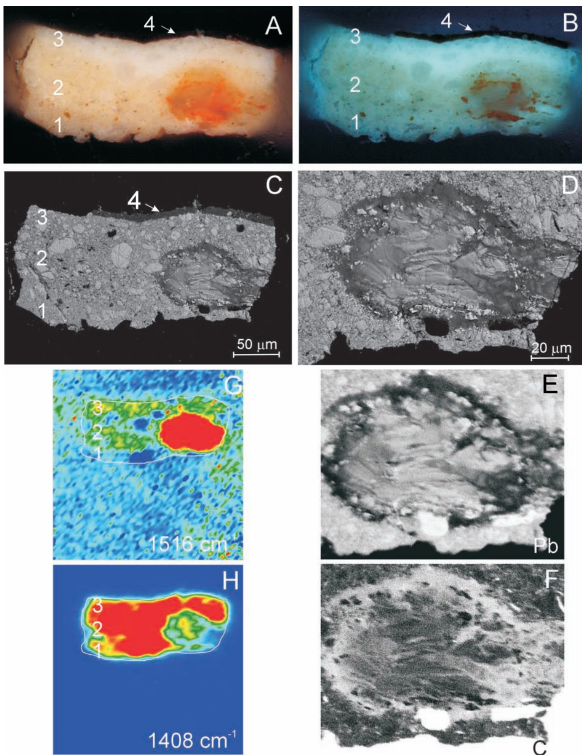
Fig. 5.4A-H Paint cross-section HSTB43/3 originating from 'Herald' (south-west) by Christiaan van Couwenbergh (1651) is depicted in the light microscopic images, white light (A) and UV (B), and in the corresponding BSE-image (C). BSE-image (D) and X-ray maps of lead (PbM) (E) and carbon (CK) (F) reveal the large lead soap aggregate. Lead carboxylates are detected and imaged with FTIR at 1516 \text{cm}^{-1} (G) and carbonates at 1408 \text{cm}^{-1} (H) (see coloured version at the end of this thesis).
