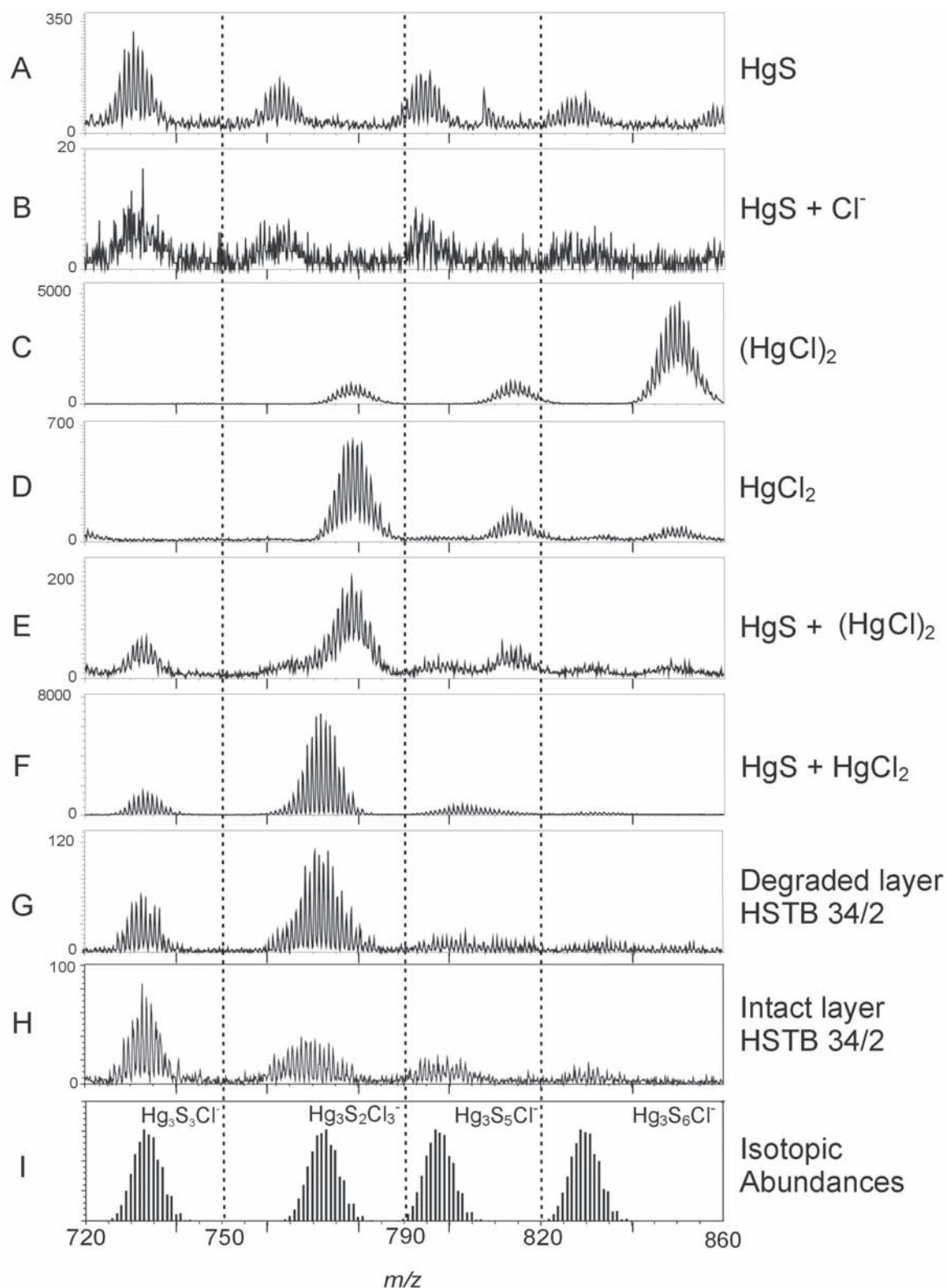
Fig. 4.6 Part of the negative ion mass spectrum in the mass window from 720–860 amu of pure \text{HgS} (A), \text{HgS} + \text{Cl}^- ions (B), pure (\text{HgCl})_2 (C), pure \text{HgCl}_2 (D); a mixture of \text{HgS} + (\text{HgCl})_2 (E); mixture of \text{HgS} + \text{HgCl}_2 (F) and paint cross-section HSTB 34/2 (G). The vertical dotted lines divide the spectra into four mass ranges which correspond with the columns in Table 4.1.
